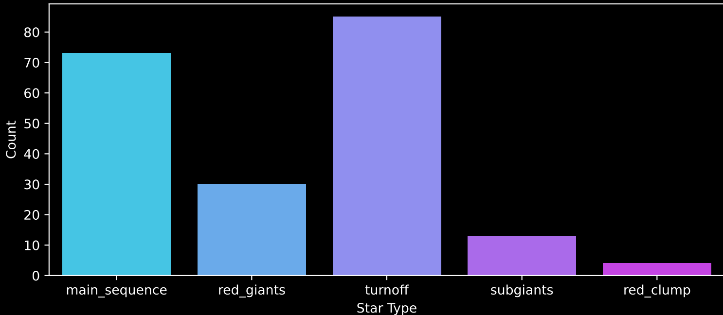
GALAH DR4 Field: [1263] Count plot of Star Type
