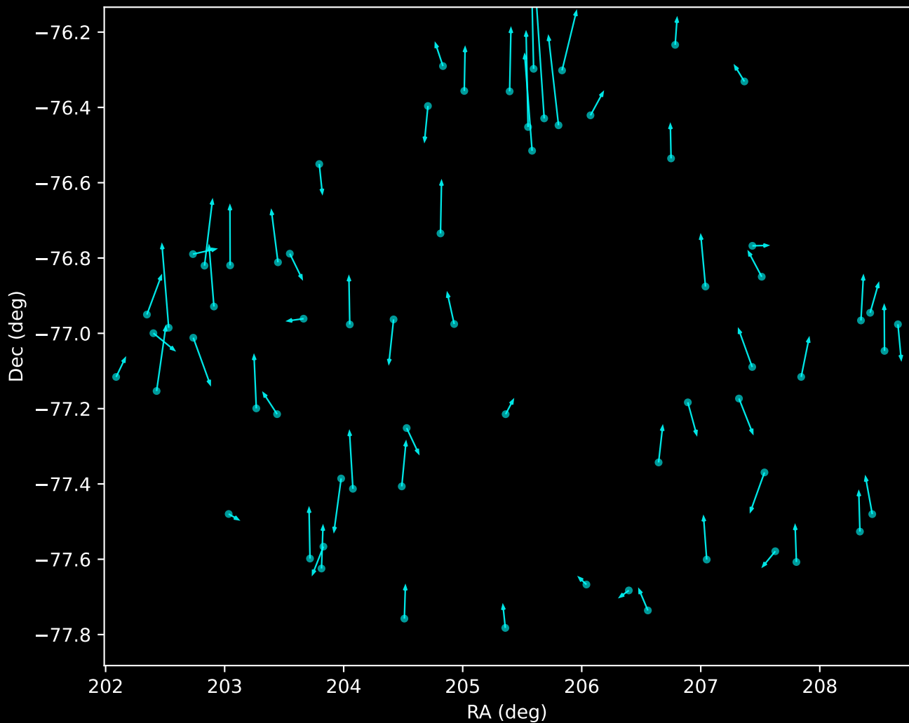
GALAH DR4 Noise Stream Proper Motion Vectors (n=66)
