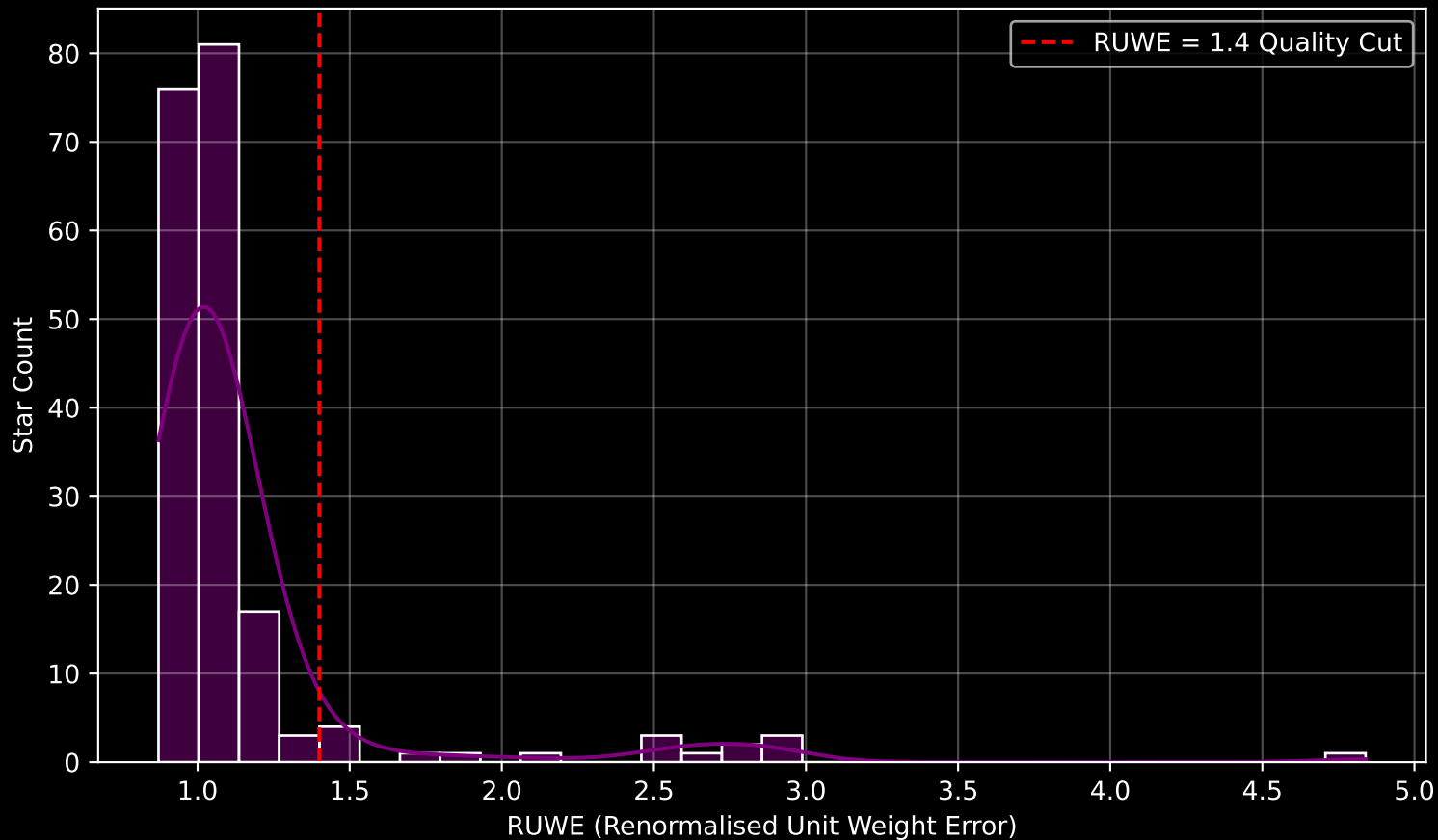
GALAH DR4 Field [1263] RUWE Distribution (n= 194)
