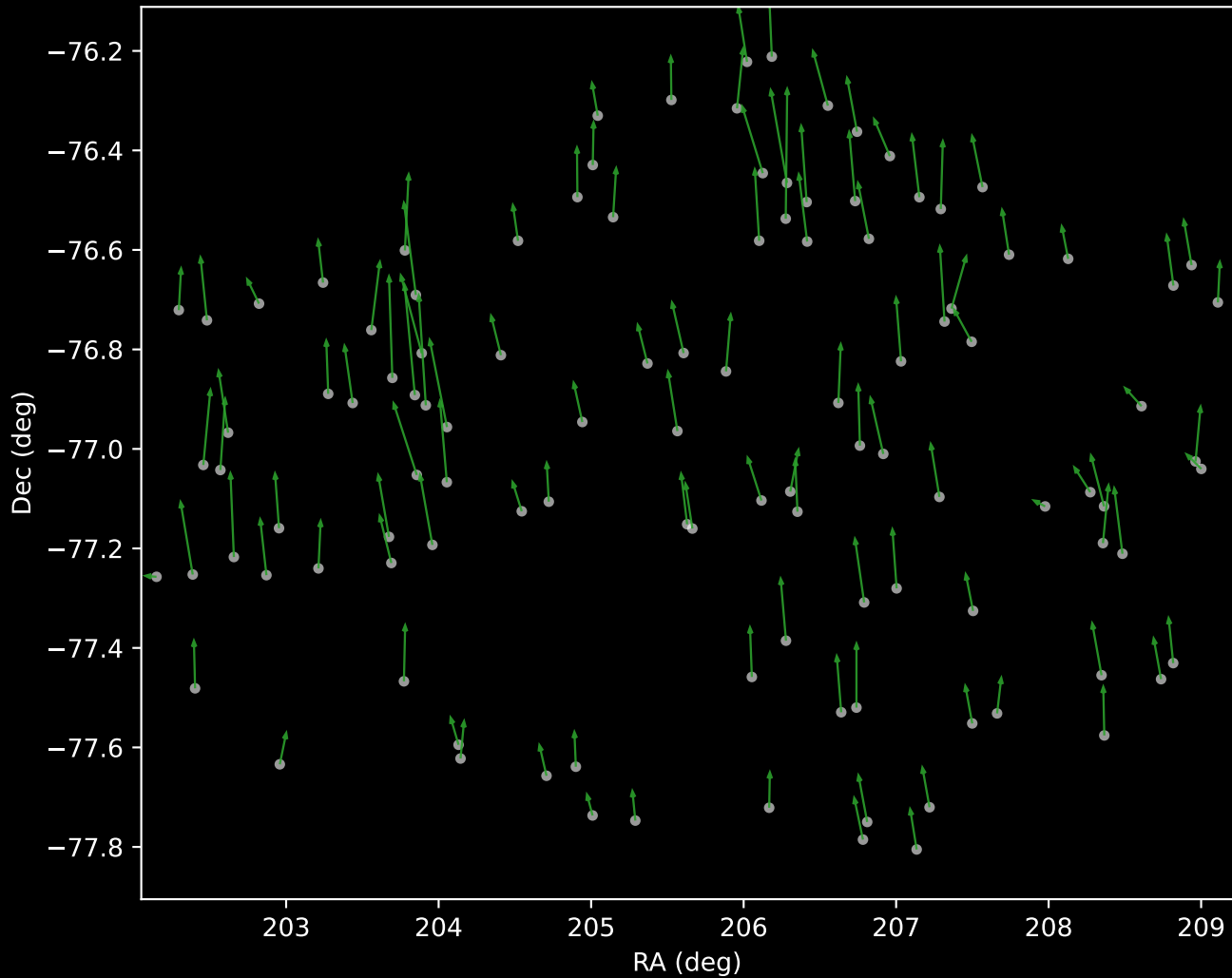
GALAH DR4 Cluster 4 Proper Motion Vectors (n=112)
